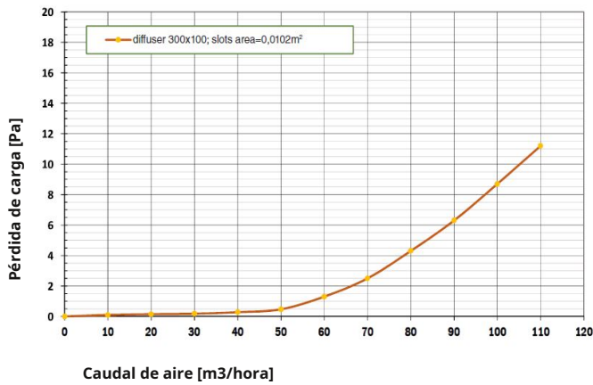
Difusor300x100
