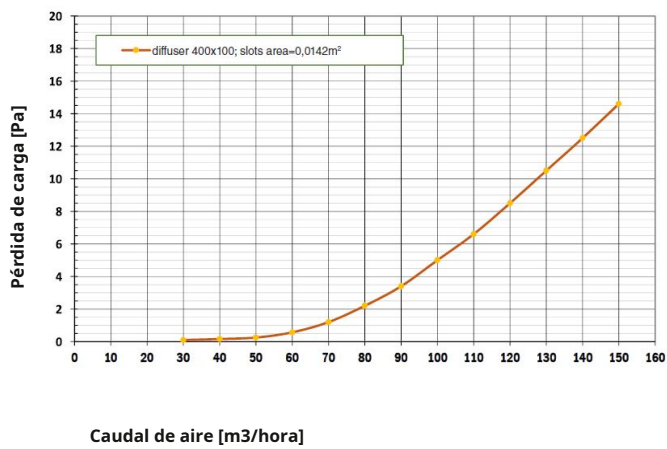
Difusor 400x100
