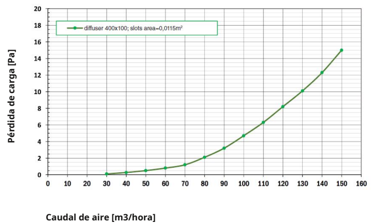
Difusor 400x100
